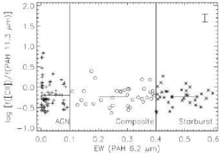
Fig 3-1. Ratio of [C II] 158 \mu\text{m} to PAH 11.3 \mu\text{m} line fluxes, compared to the source classification from EW(PAH 6.2 \mu\text{m} )
